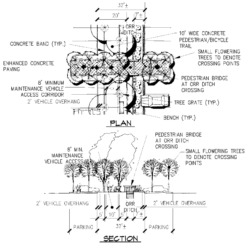
Exhibit 10-6 Orr Ditch Trail Cross Section
