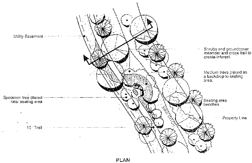
Exhibit 10-2 Orr Ditch Residential Plan
