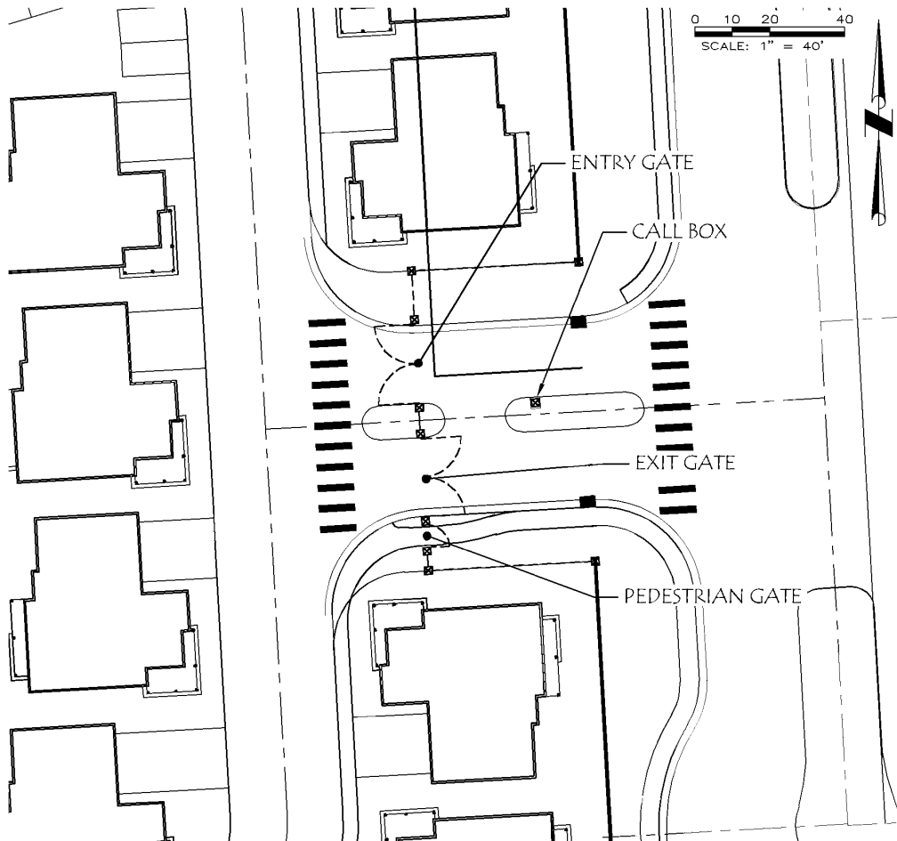
Exhibit 5.3-3 Primary Entry
