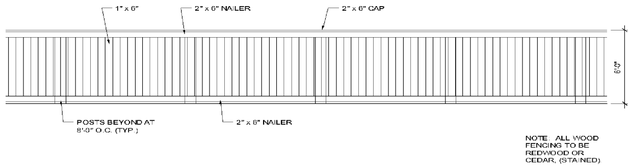
VILLAGE FENCE - TYPE 2
