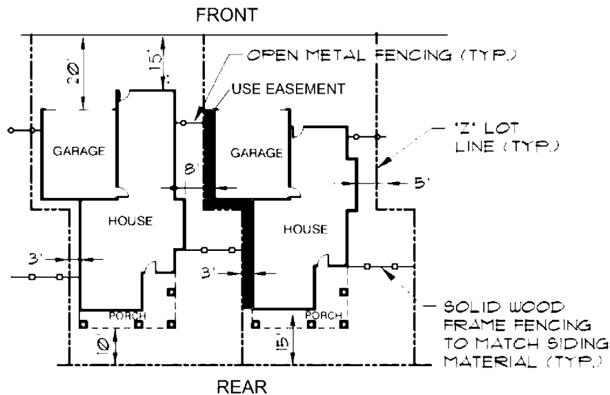
Exhibit 5.2-2 Typical "Z Lot" Setback Configuration
