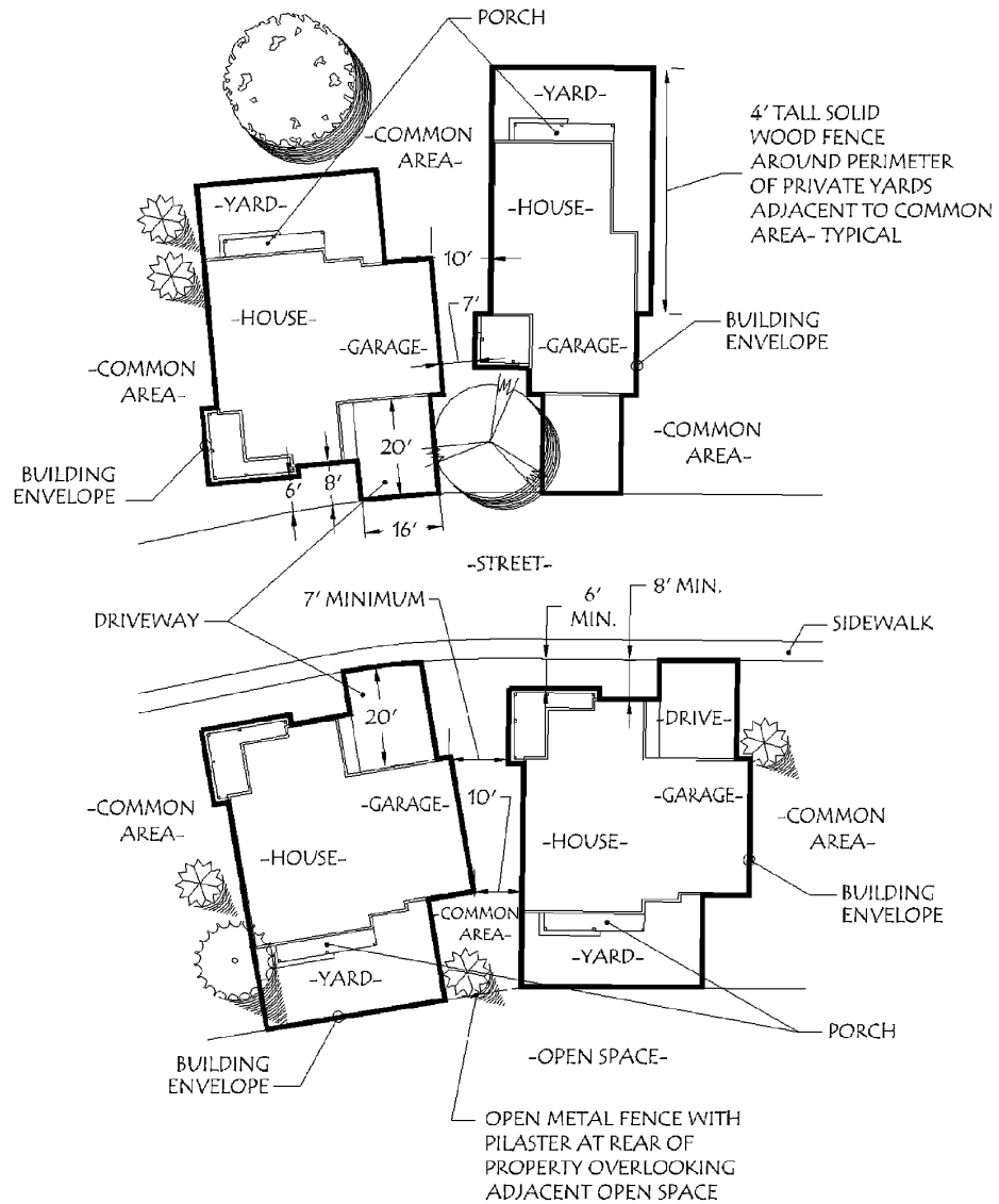
Exhibit 5.3-2 Typical Cottage Homes Lot Setback Configuration
